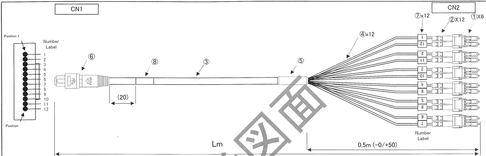
(Sheet A) Cable Performance specification
