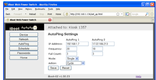
AutoPing Setup Page
